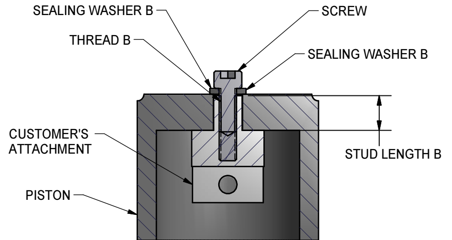
SECTION B-B SCALE 3
